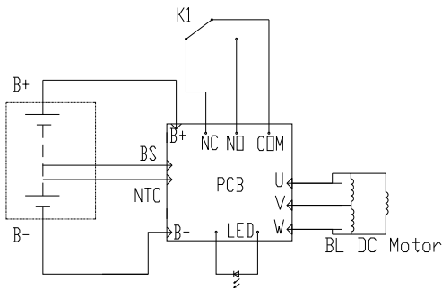
Electric circuit
