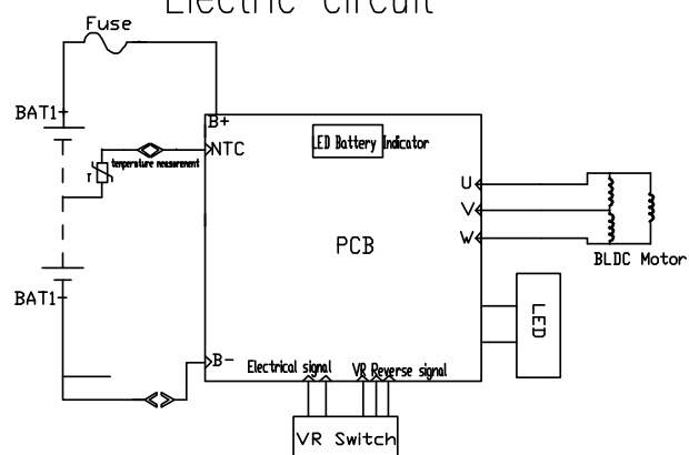
Electric circuit
