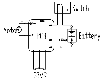
Electric circuit
