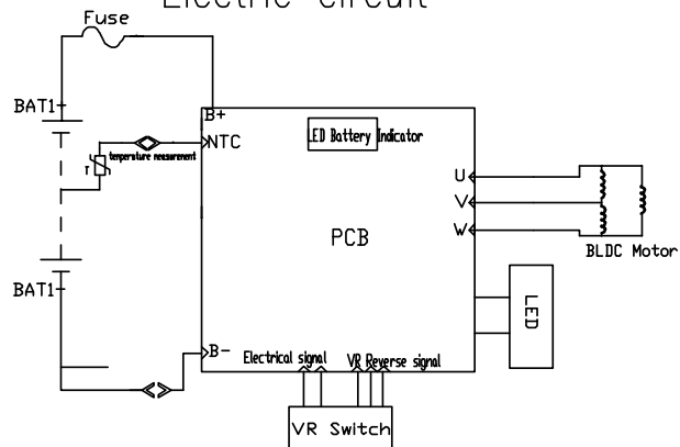
Electric circuit
